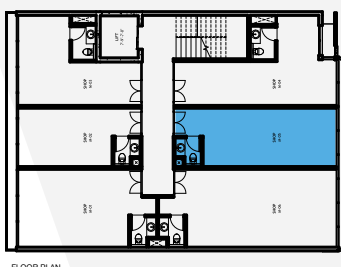
FLOOR PLAN
